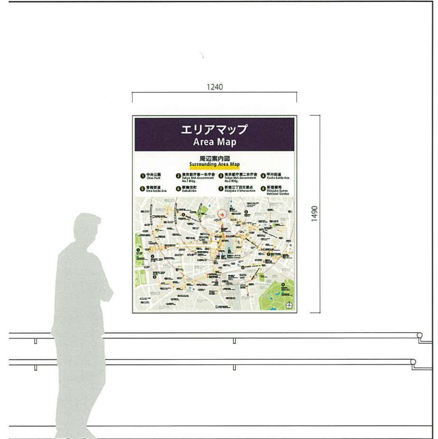
T-図05 器具外形寸法H1490×W1240
